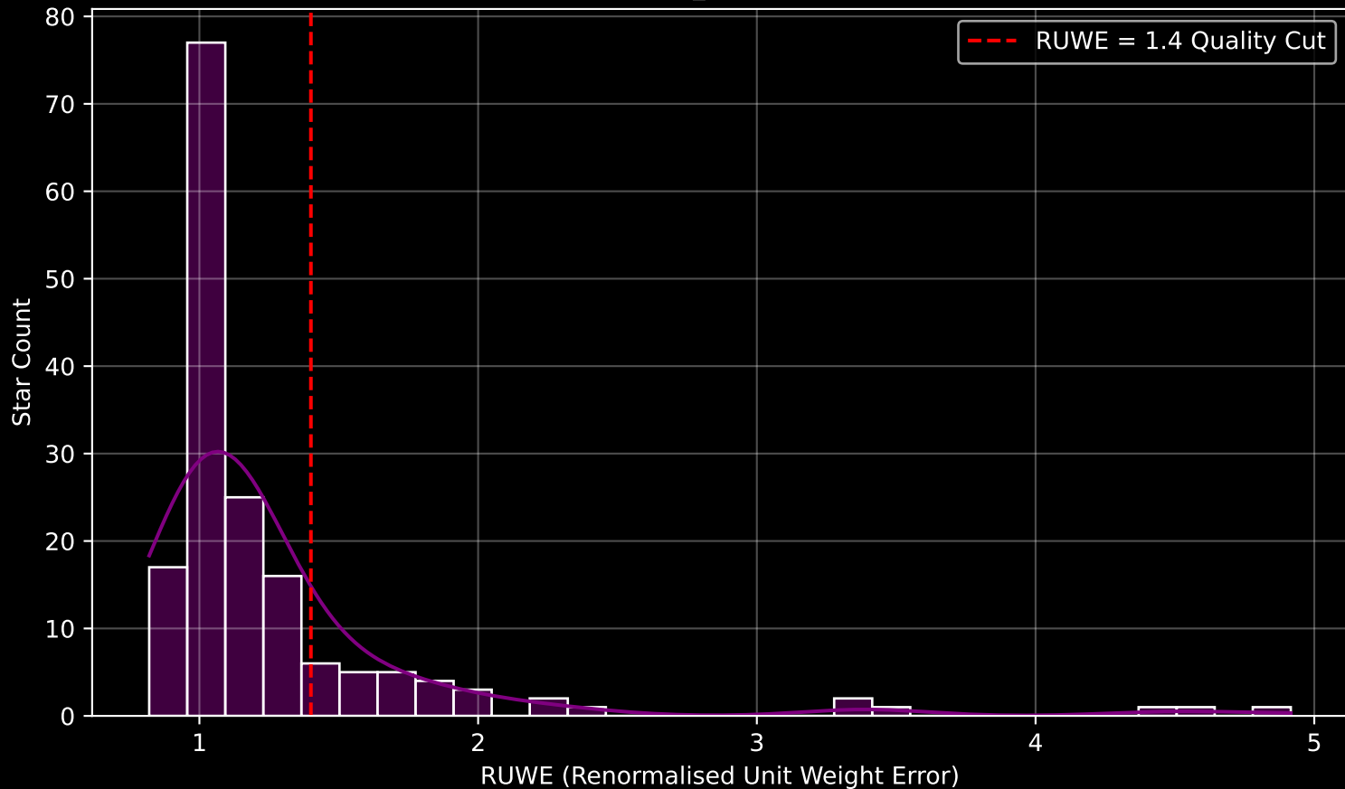
GAPOGEE DR17 Field [232+34_MGA] RUWE Distribution (n= 167)
