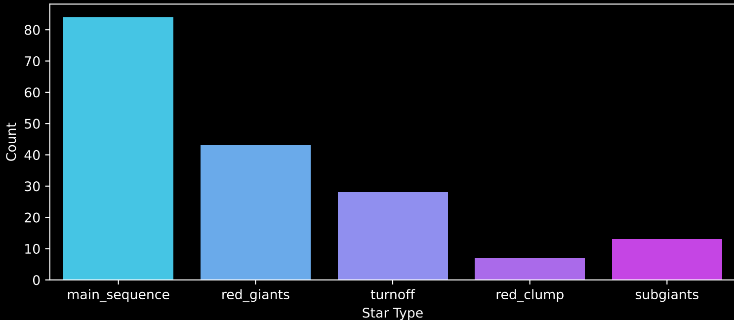
APOGEE DR17 Field: [232+34_MGA] Count plot of Star Type
