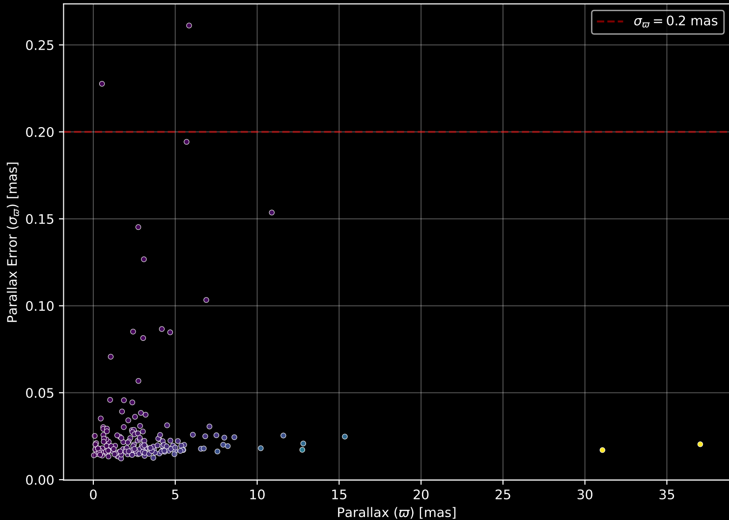
APOGEE DR17 Field: [232+34_MGA] Parallax Quality (n= 175)
