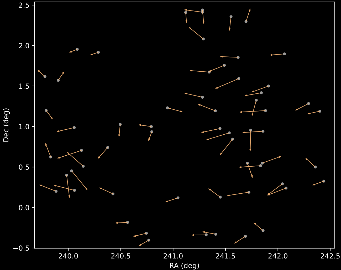
APOGEE DR17 Cluster 3 Proper Motion Vectors (n=60)
