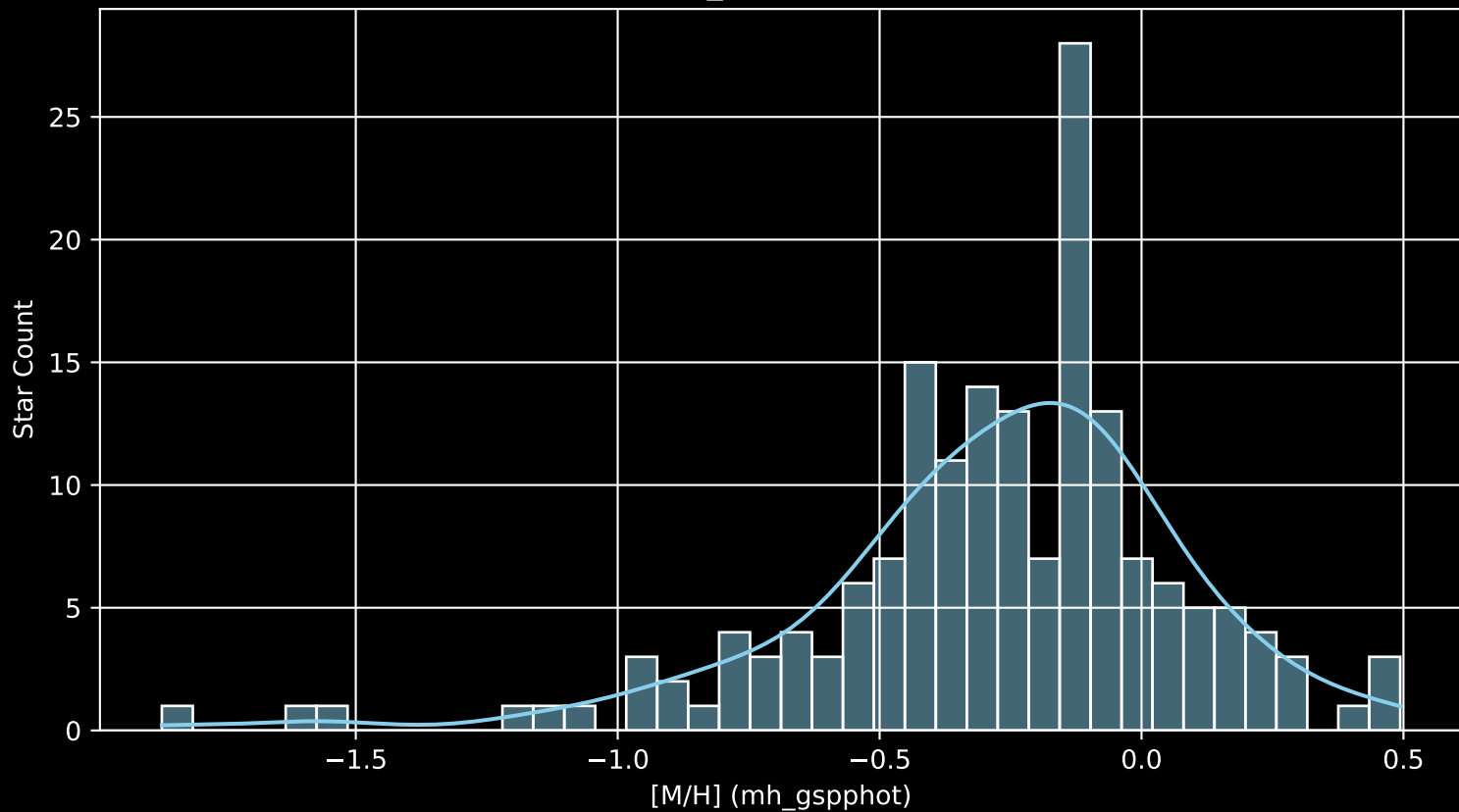
APOGEE DR17 Field: [232+34_MGA [M/H] (mh_gspphot) (n= 174)
