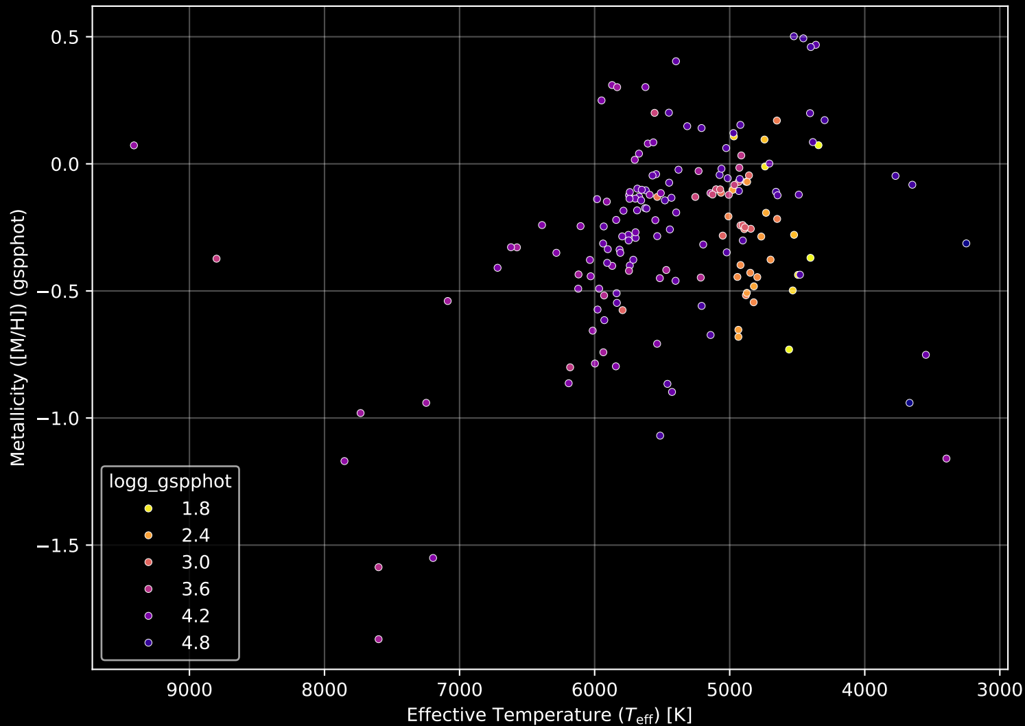
APOGEE DR17 Field: [232+34_MGA] Stellar Population Parameters (n= 175)
