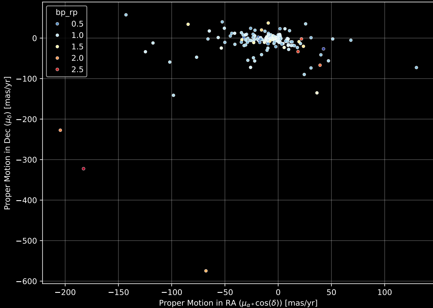
APOGEE DR17 Field: [232+34_MGA] Proper Motion Diagram (n= 175)
